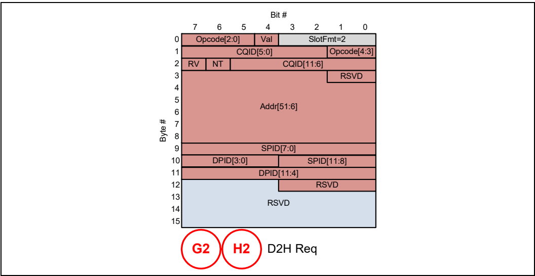
Figure 4-49. 256B Packing: G2/H2 PBR Messages
