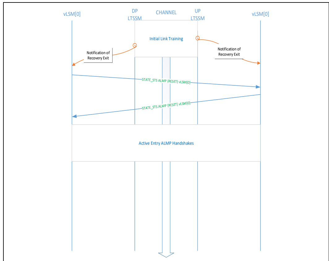
Figure 5-13. Both Upstream Port and Downstream Port Notify ARB/MUX of Recovery Transitions
