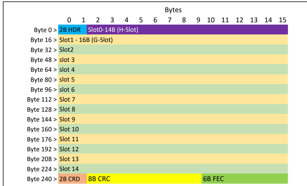
Figure 4-41. Standard 256B Flit
