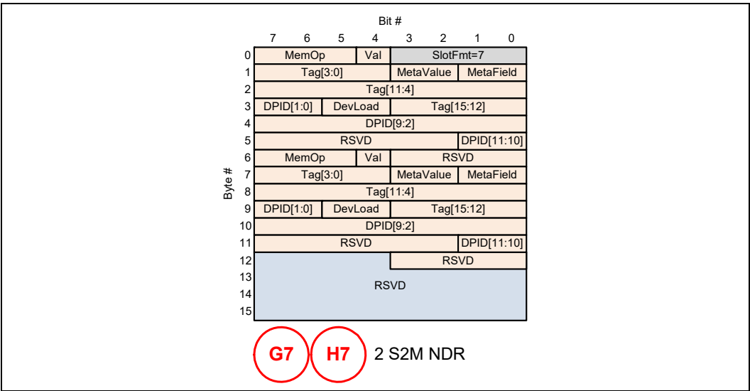
Figure 4-59. 256B Packing: G7/H7 PBR Messages
