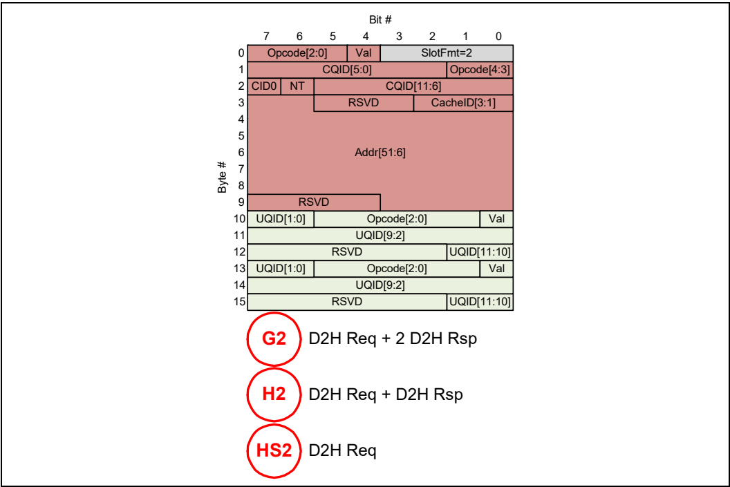
Figure 4-49. 256B Packing: G2/H2 PBR Messages
