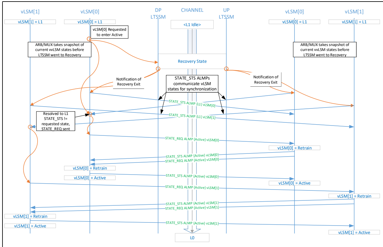
Figure 5-11. CXL Exit from PM State Example
