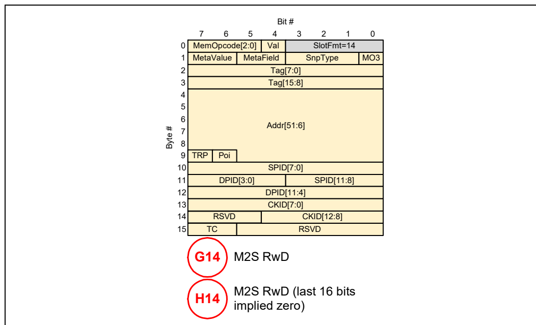
Figure 4-65. 256B Packing: G14/H14 PBR Messages
