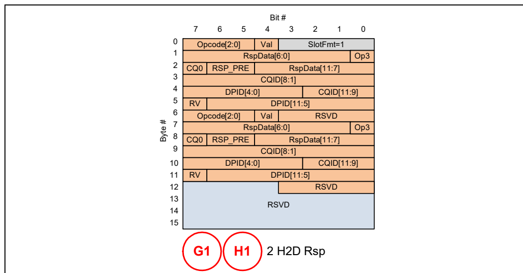
Figure 4-47. 256B Packing: G1/H1 PBR Messages
